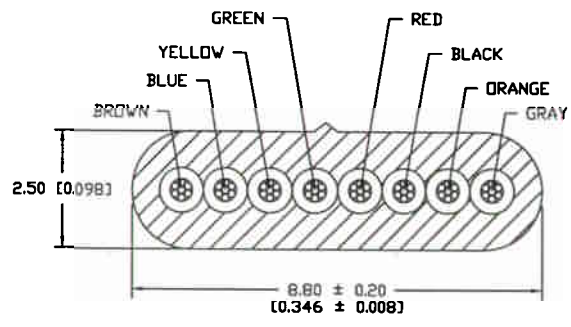
8 CONDUCTOR CABLE
