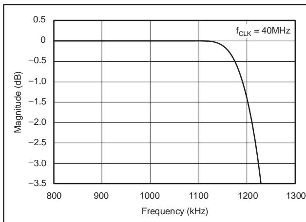
Figure 50. Passband Transition
