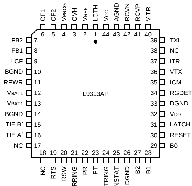
Figure 2. 44-Pin PLCC
