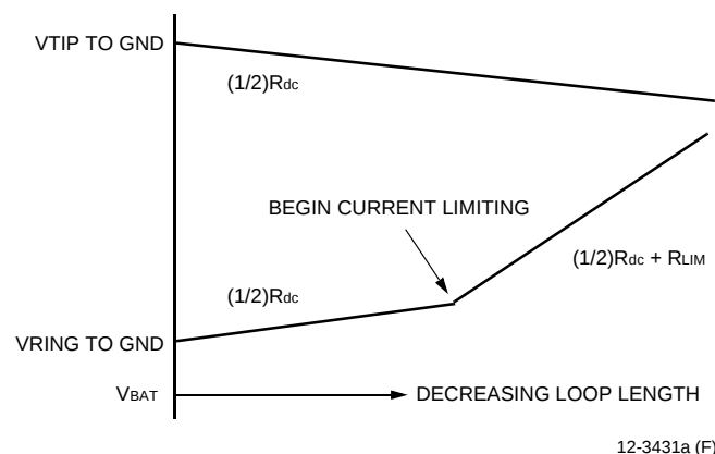
Figure 12. Tip/Ring Voltage
