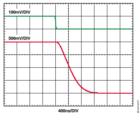
Figure 9. Fall Time
