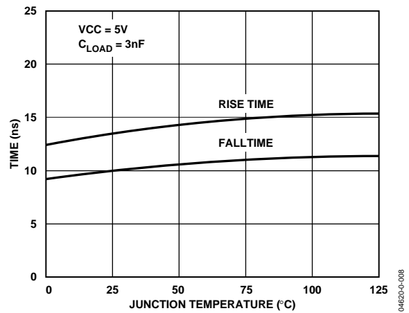
Figure 9. DRVH Rise and Fall Times vs. Temperature
