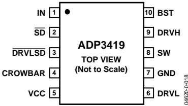
Figure 5. Pin Configuration
