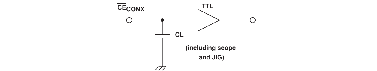
Figure 1. Output Load
