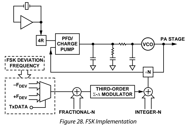
Figure 28. FSK Implementation
