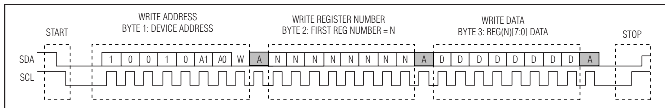
Figure 22. I 2 C Single Register Write Sequence
