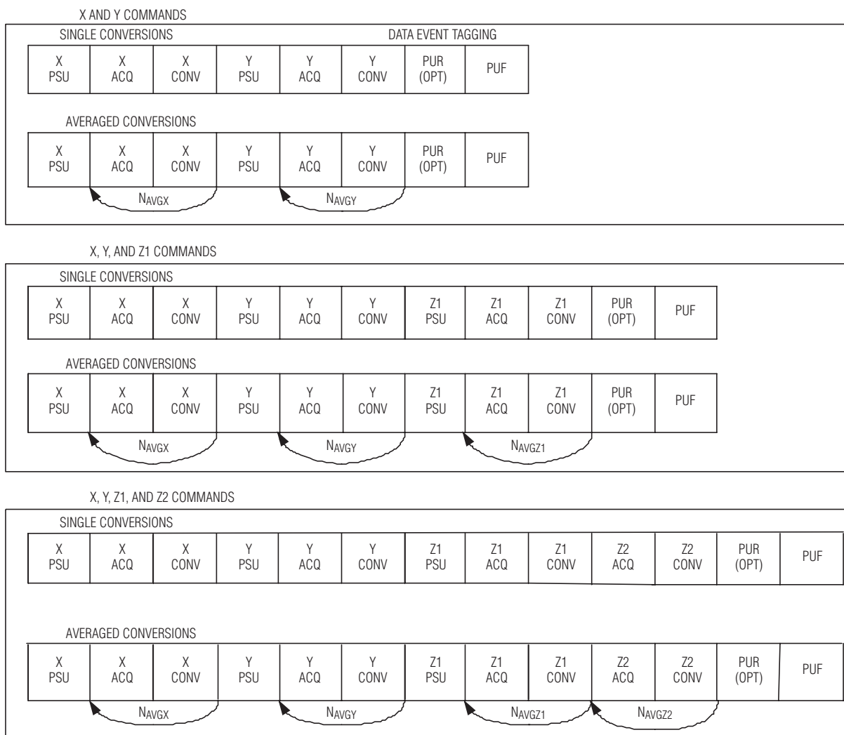
Figure 13. Combined Commands
