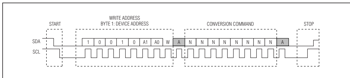
Figure 26. I 2 C Conversion Command
