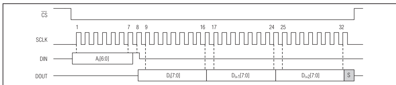
Figure 20. SPI Multiple-Byte Register Read Sequence
