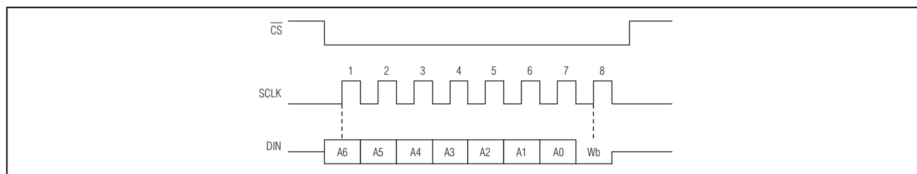
Figure 21. SPI Conversion Command
