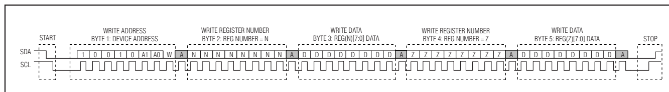
Figure 23. I 2 C Multiple Register Write Sequence
