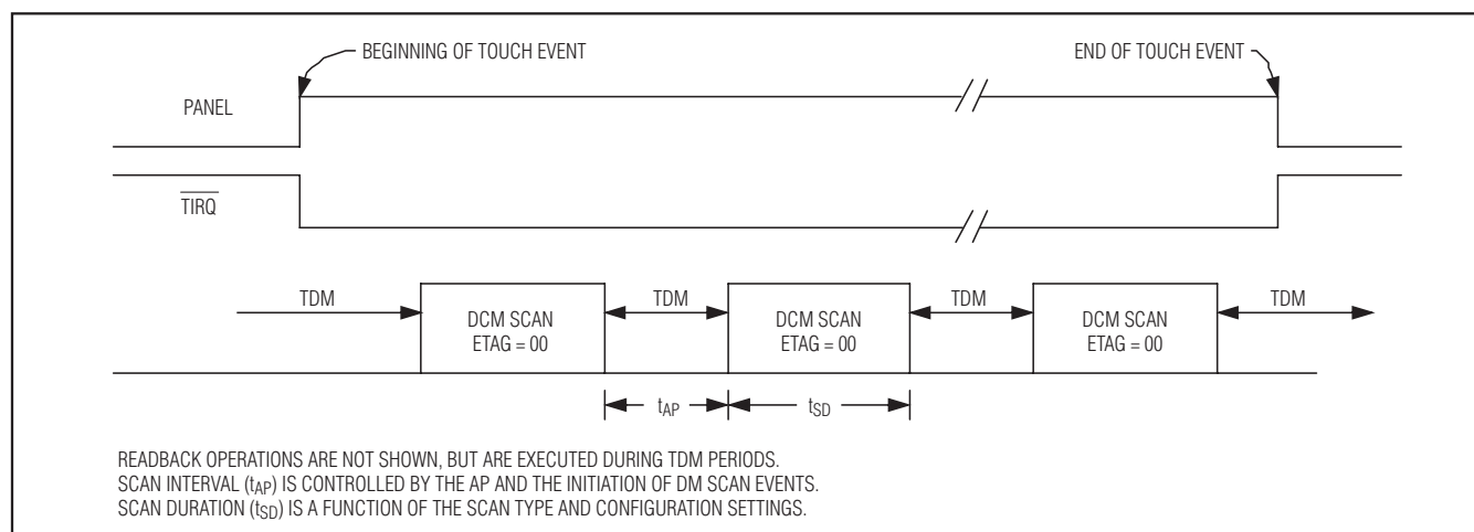
Figure 9. Continuous Interrupt Mode (Direct Conversion Mode)
