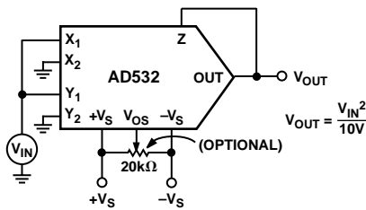
Figure 12. Squarer Connection
