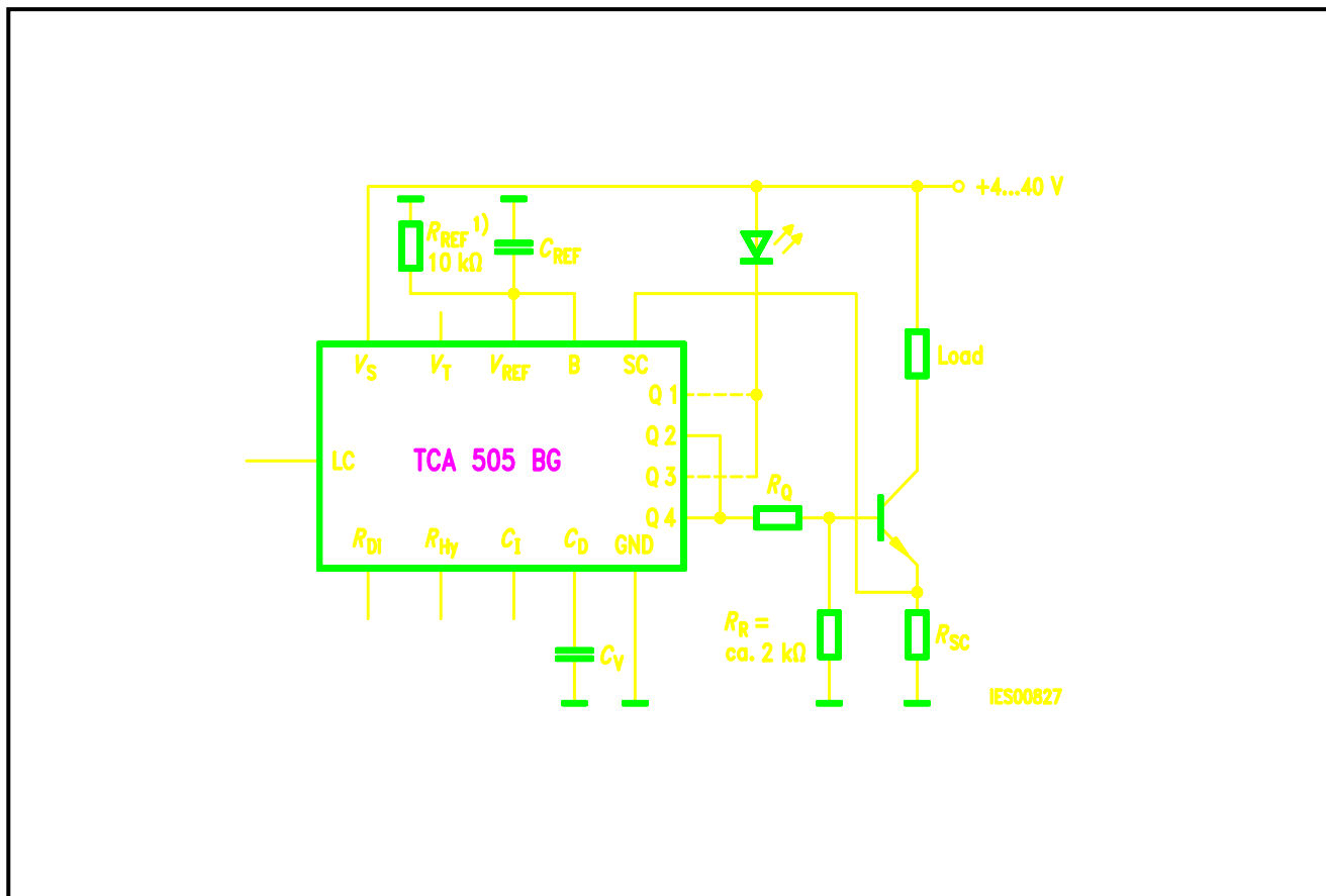
Application Circuit 3
