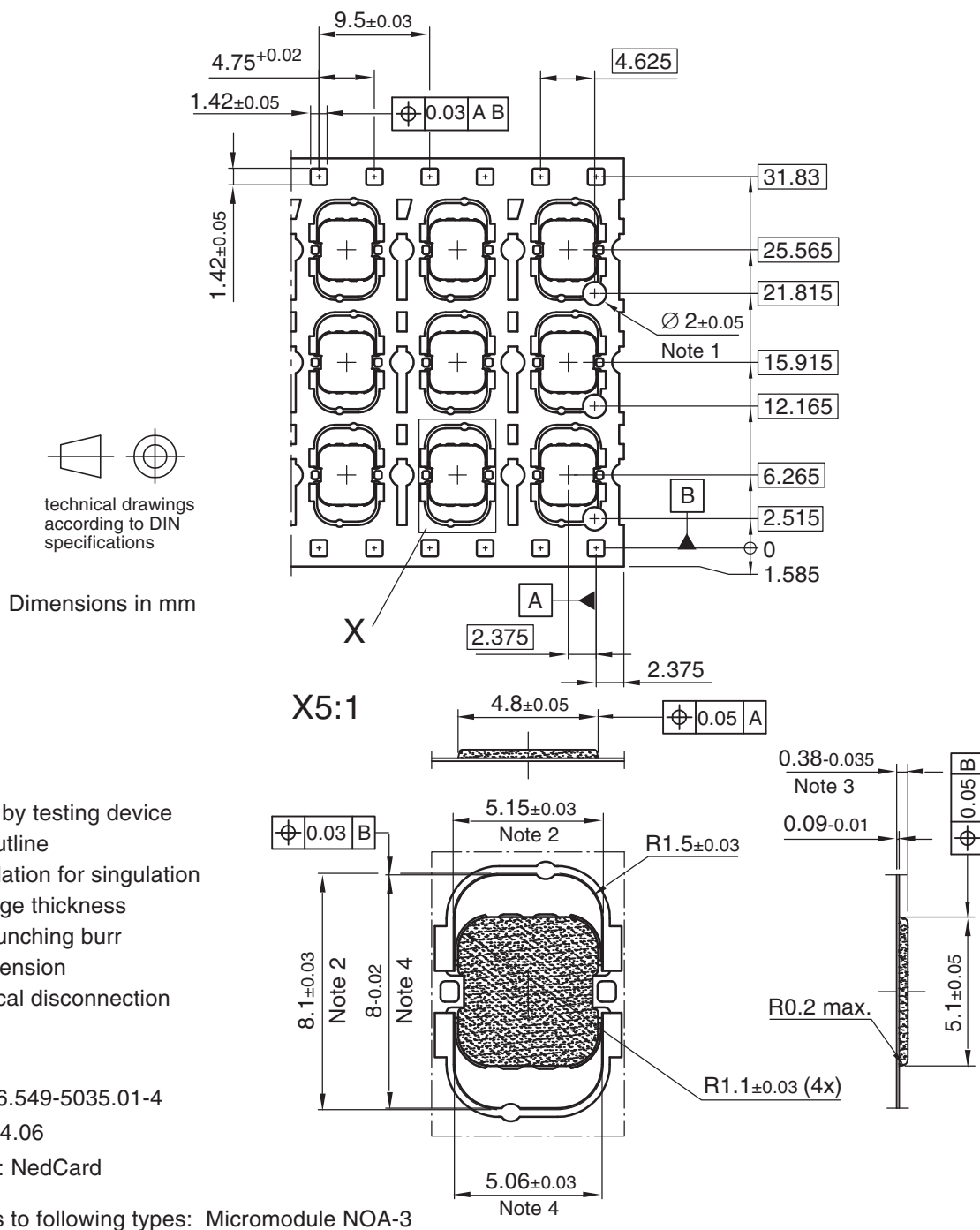
Figure 10-5. NOA3 Micromodule
