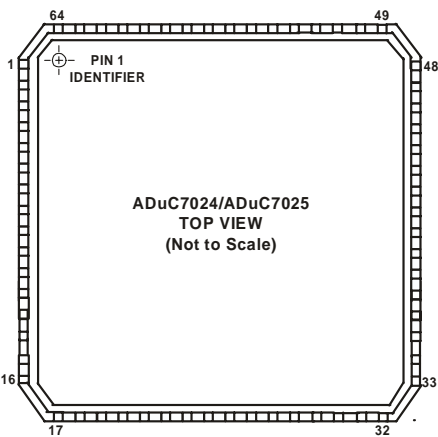
64-Lead CSP
