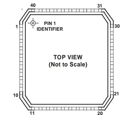
40-Lead CSP
