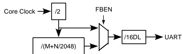
Figure 26: baudrate generation options
