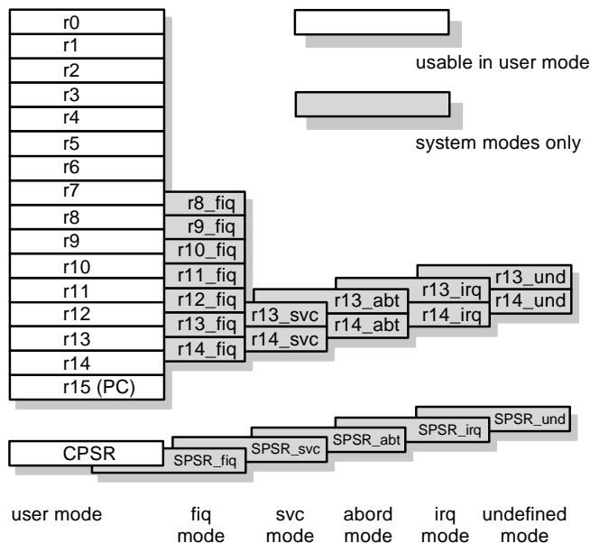
Figure 3: register organisation
