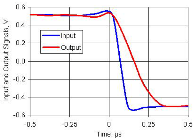
Figure 11-30. Opamp Step Response, Falling
