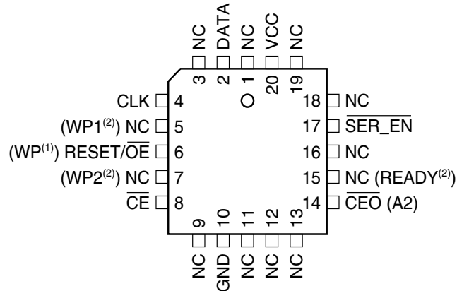
Figure 2-4. 20-lead PLCC
