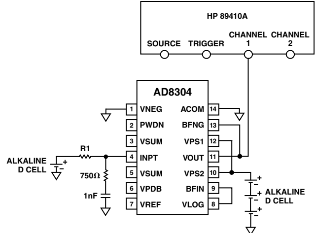
Figure 21. Configuration for Noise Spectral Density Measurement
