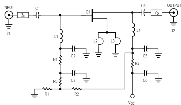
Figure 23. Typical ATF-54143 LNA with Passive Biasing.
