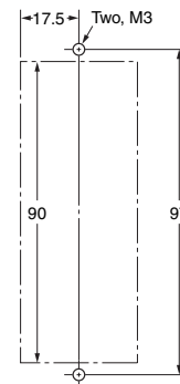
Mounting Hole Dimensions
