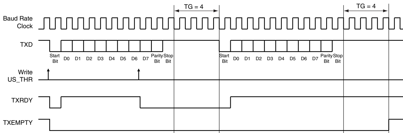
Figure 33-23. Timeguard Operations
