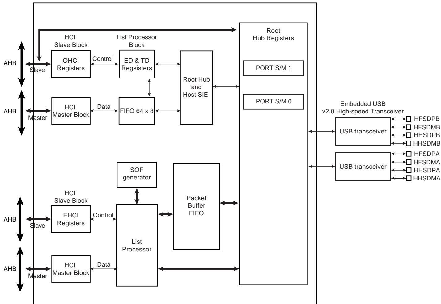
Figure 37-2. Block Diagram
