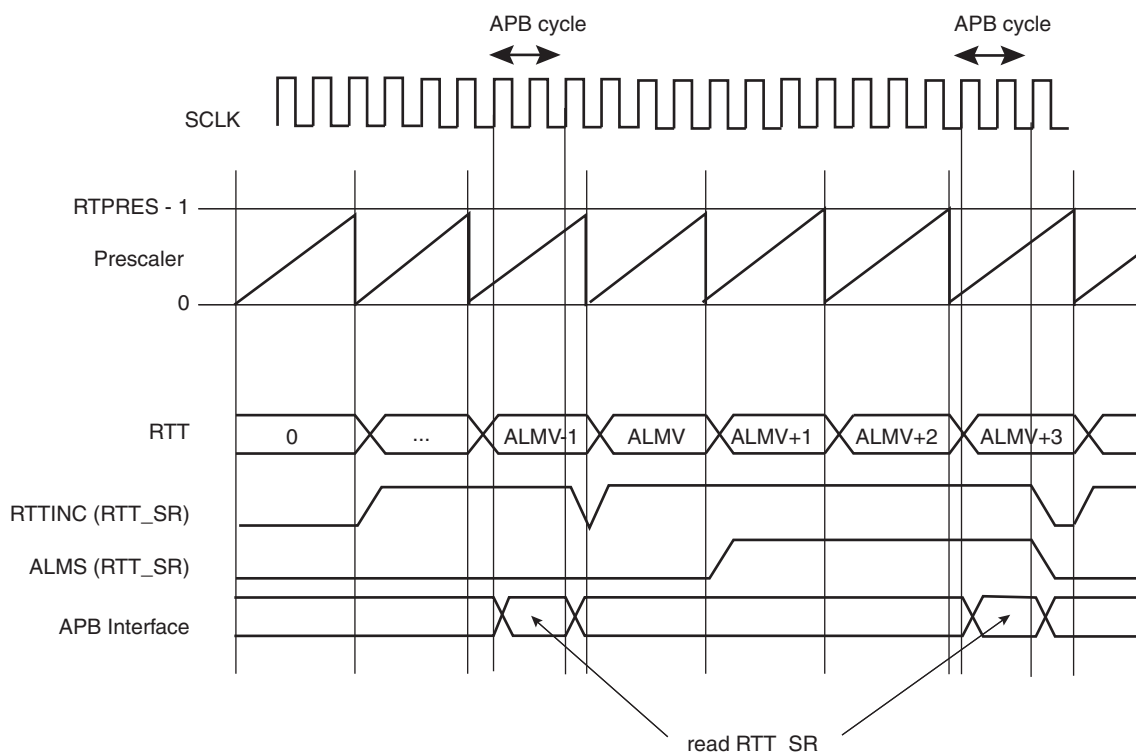
Figure 13-2. RTT Counting
