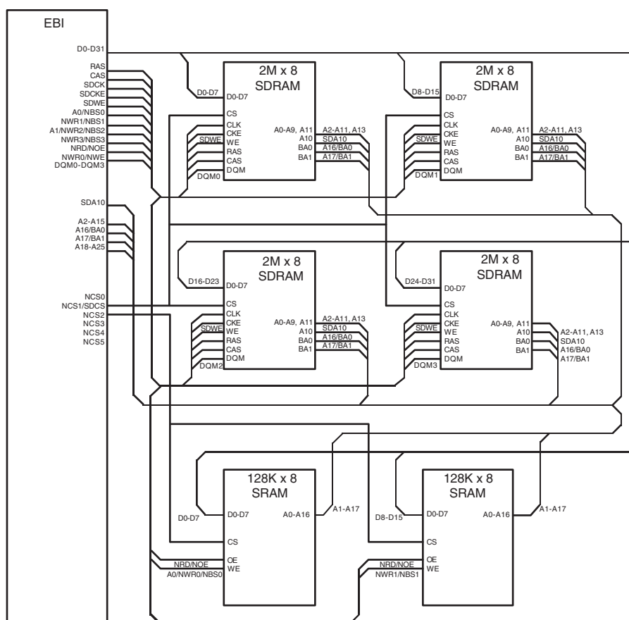
Figure 20-4. EBI Connections to Memory Devices
