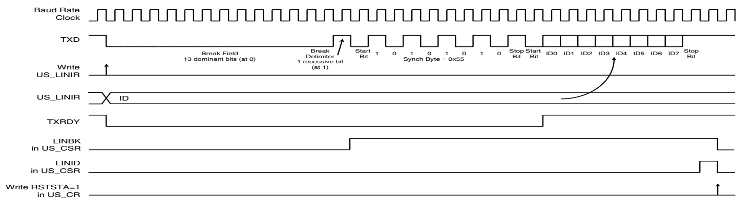
Figure 33-40. Header Transmission
