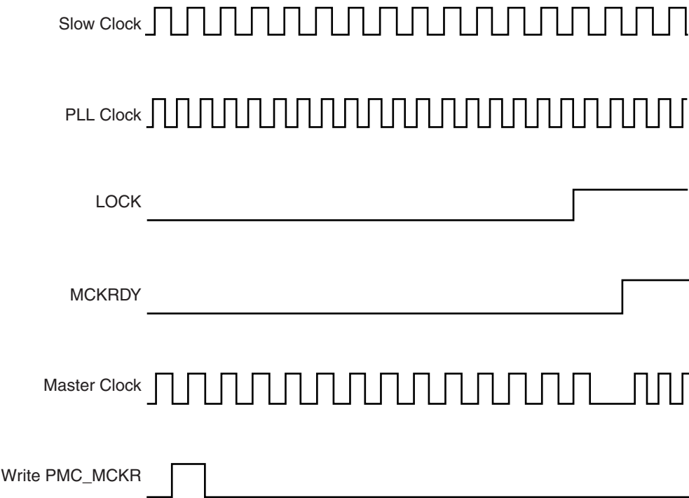
Figure 26-3. Switch Master Clock from Slow Clock to PLLA Clock
