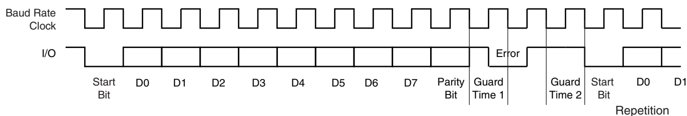
Figure 33-32. T = 0 Protocol with Parity Error
