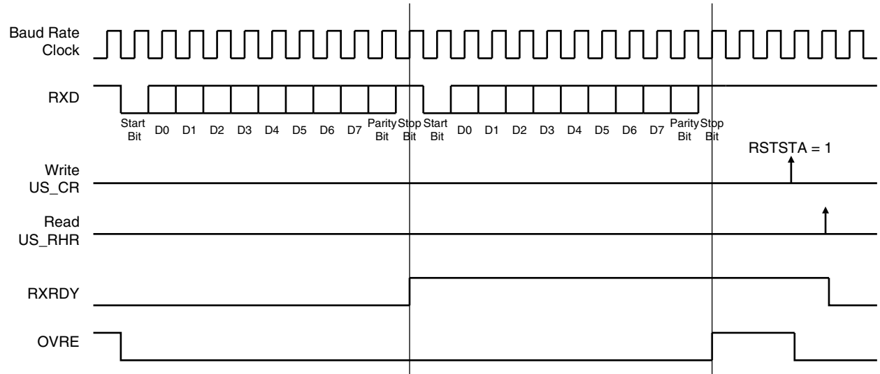
Figure 33-21. Receiver Status
