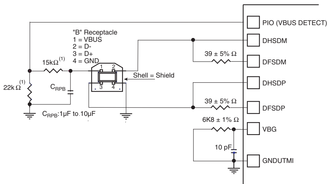
Figure 38-3. Board Schematic
