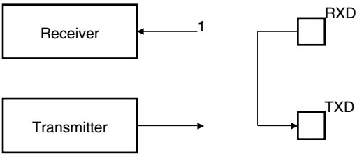
Figure 33-58. Remote Loopback Mode Configuration
