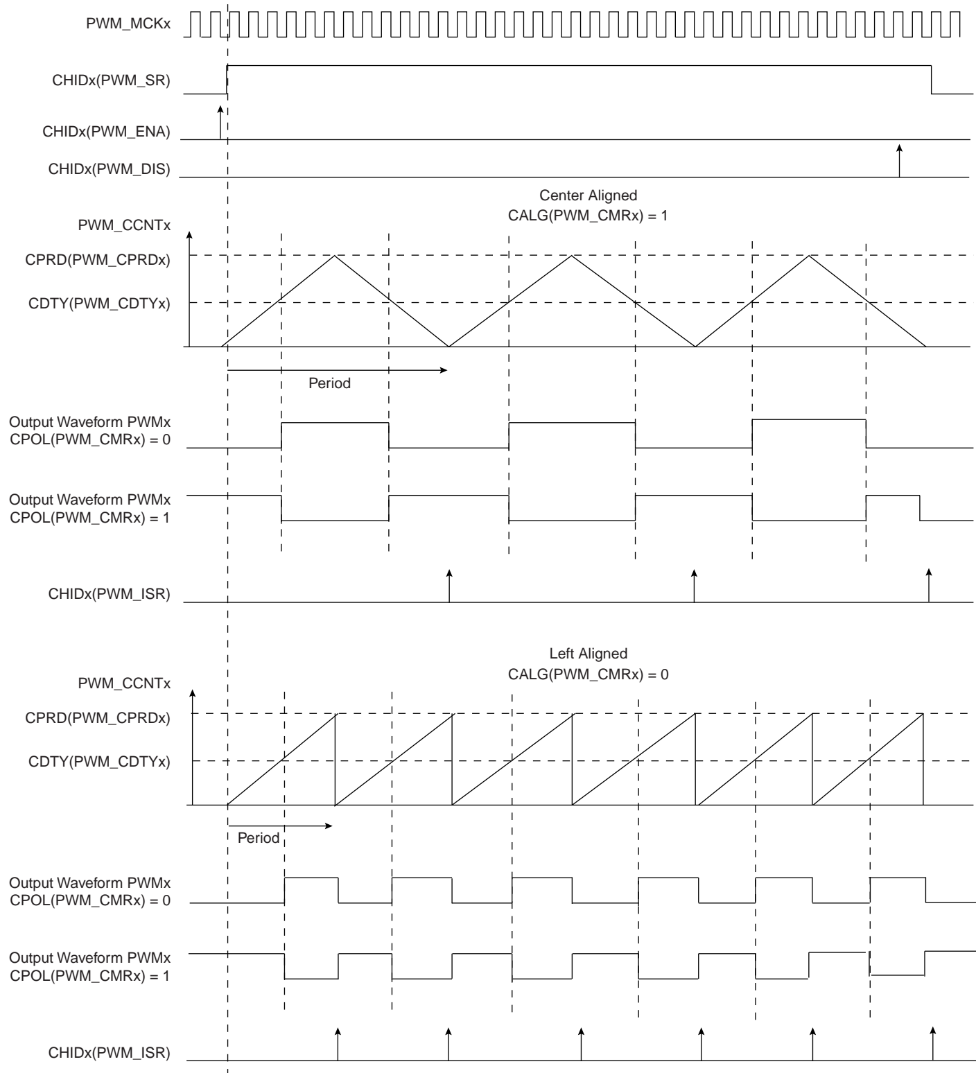
Figure 42-5. Waveform Properties
