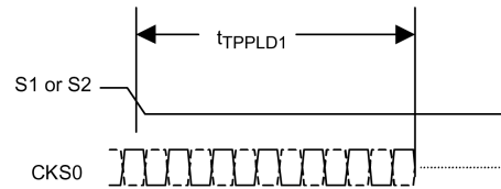
FIGURE 25. PLL Power-Down Time
