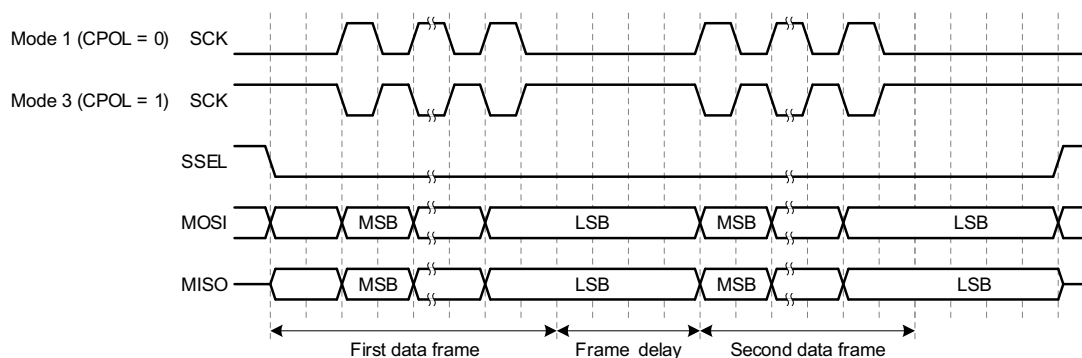
Fig 49. Frame_delay
