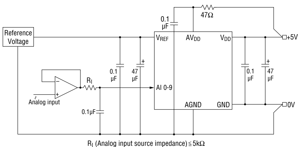
Figure 1 Recommended Circuit
