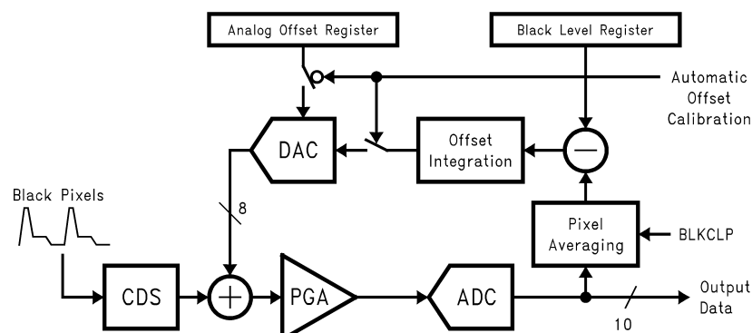
FIGURE 10. Digital Black Level Correction Loop
