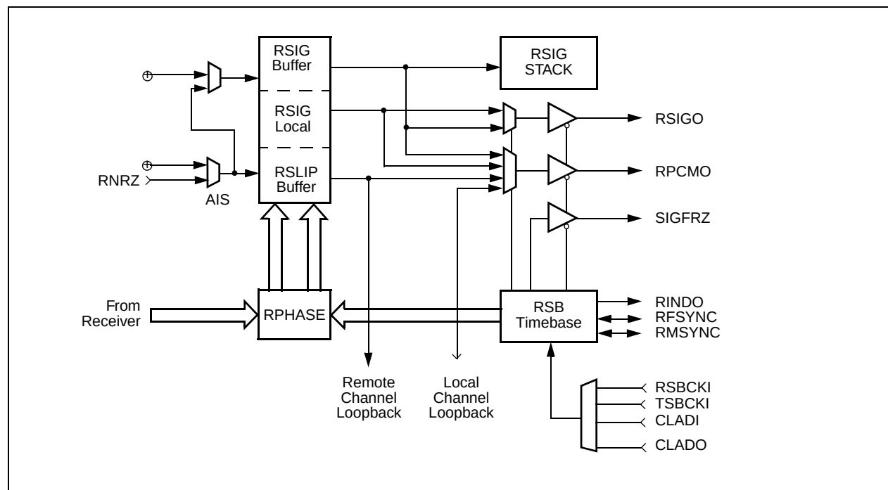
Figure 2-18. RSB Diagram
