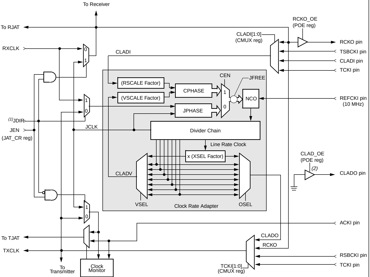
Figure 2-22. Clock Rate Adapter/Jitter Attenuator Block Diagram (B18376 Device Only)
