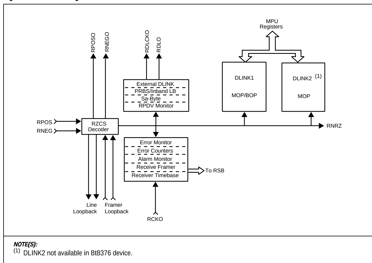
Figure 2-11. RCVR Diagram
