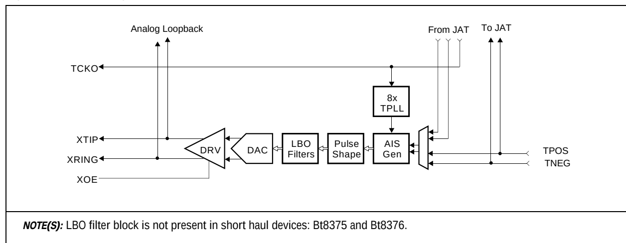
Figure 2-33. TLIU Diagram
