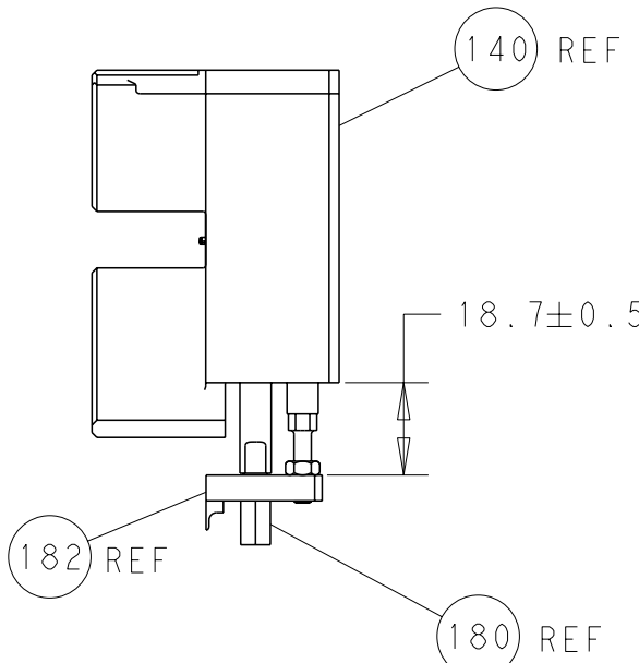
HOLDDOWN SET-UP
