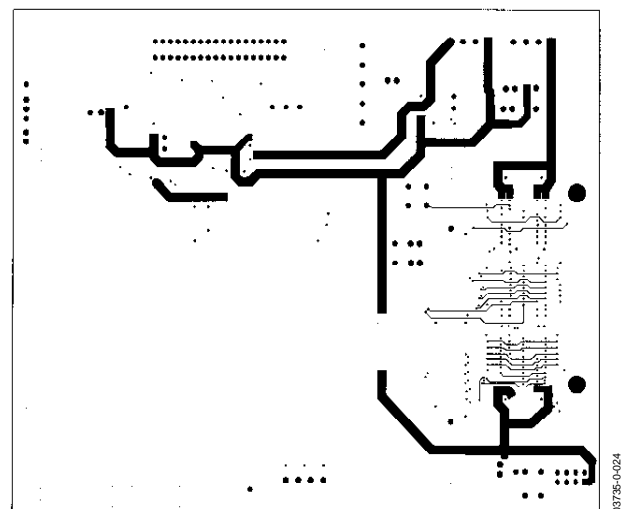
Figure 26. Power Plane 2
