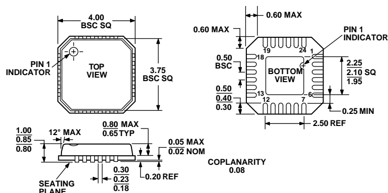
Figure 42. 24-Lead Lead Frame Chip Scale Package [LFCSP_VQ]
