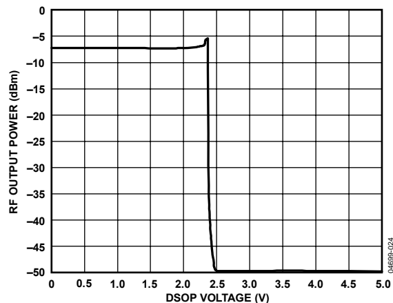
Figure 24. Power Shutdown Attenuation
