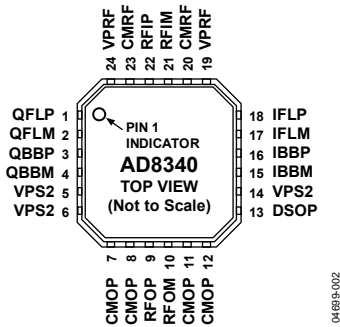
Figure 2. Pin Configuration
