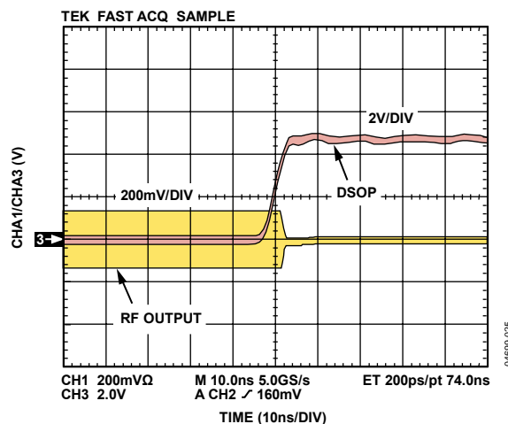
Figure 25. Power Shutdown Response Time
