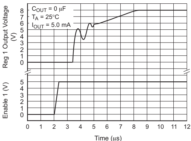
Figure 14. Regulator 1 Startup
