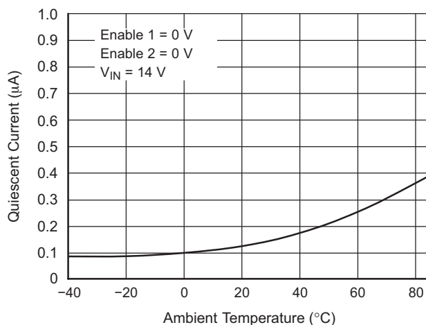
Figure 9. Quiescent Current
