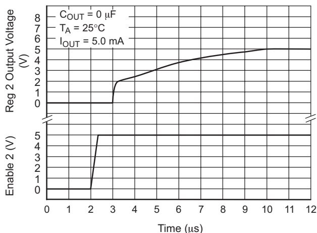
Figure 15. Regulator 2 Startup
