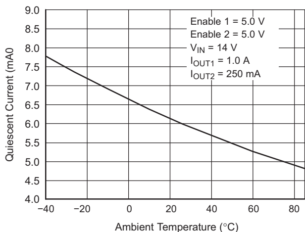
Figure 8. Quiescent Current
