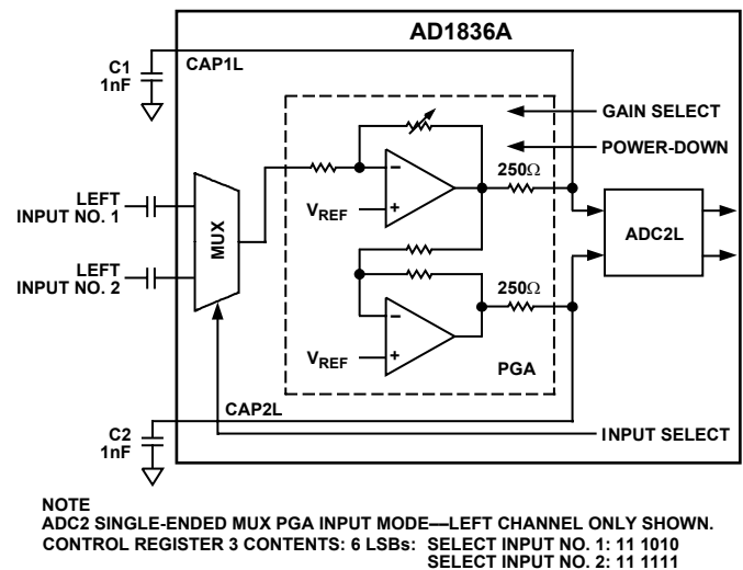
Figure 13. Single-Ended MUX/PGA Mode
