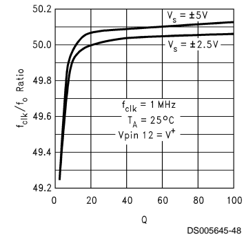
f_{\text{CLK}}/f_0 Ratio vs Q
