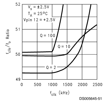
f_{\text{CLK}}/f_0 Ratio vs f_{\text{CLK}}
