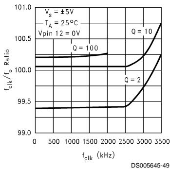
f_{\text{CLK}}/f_0 Ratio vs f_{\text{CLK}}
