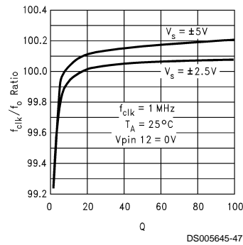
f_{\text{CLK}}/f_0 Ratio vs Q
