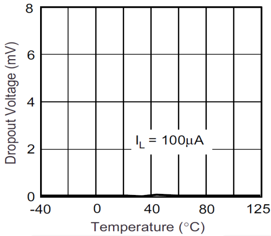
Figure 21. Dropout Voltage
