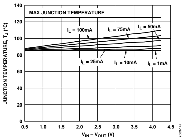
Figure 47. WLCS, T_B = 85^\circ\text{C}
