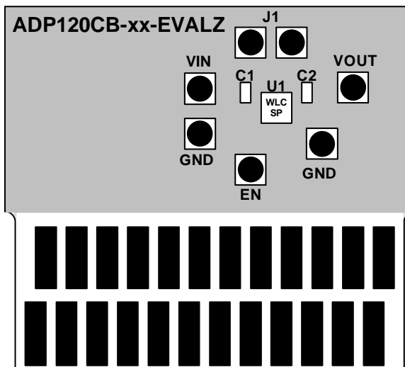
Figure 49. WLCS PCB Layout
