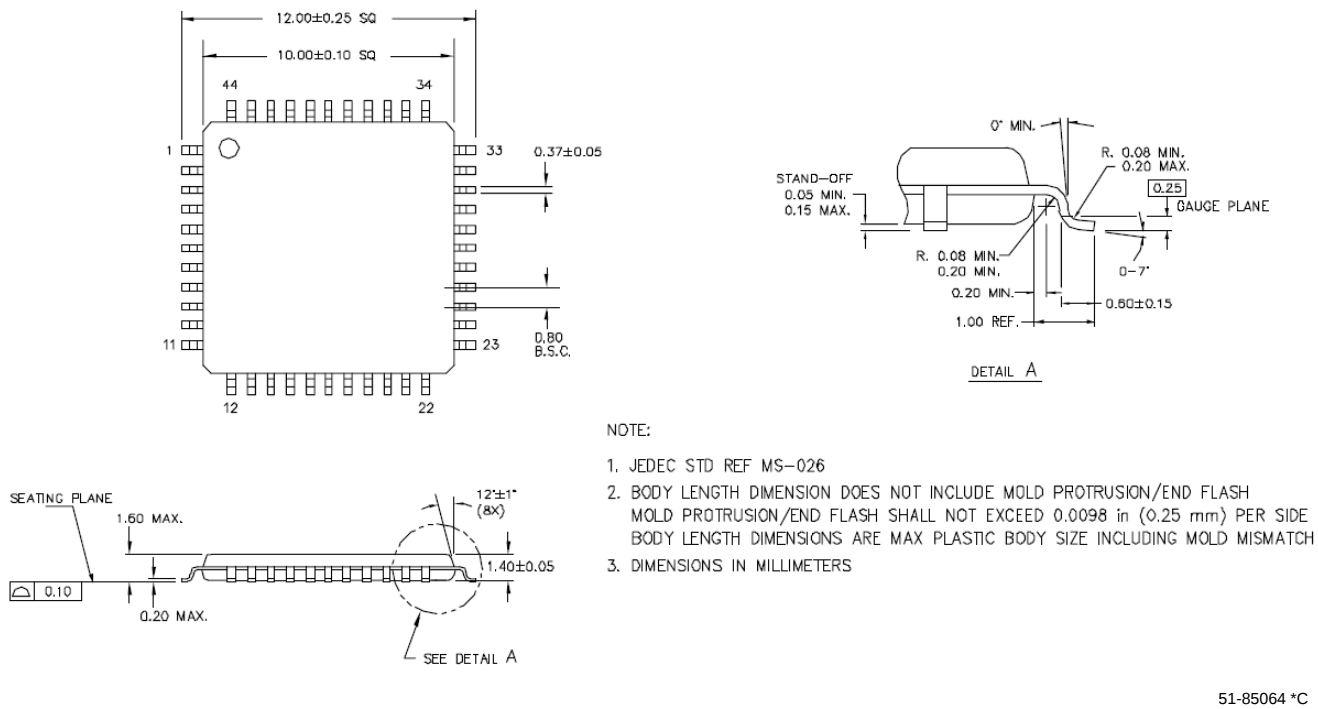
Figure 4-7. 44-Lead TQFP
