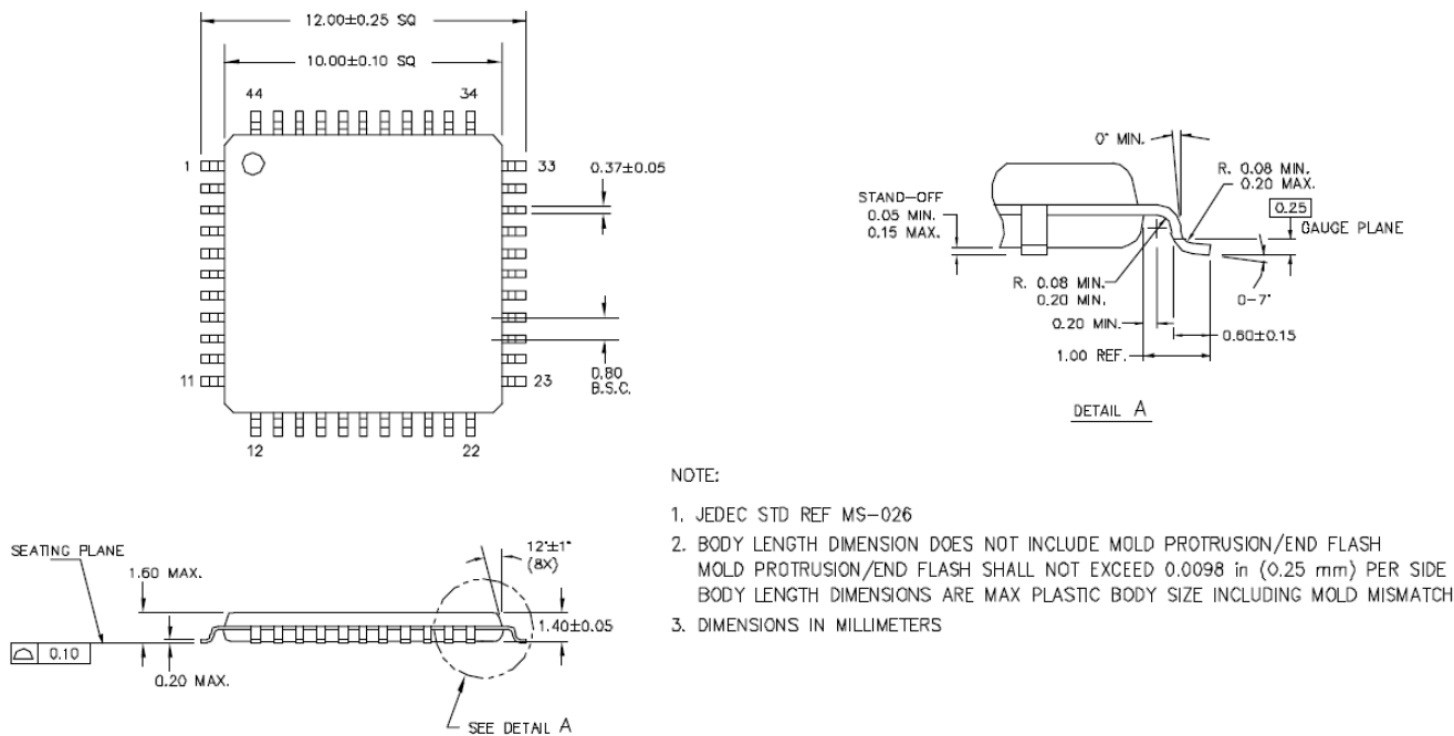
Figure 4-7. 44-Lead TQFP
