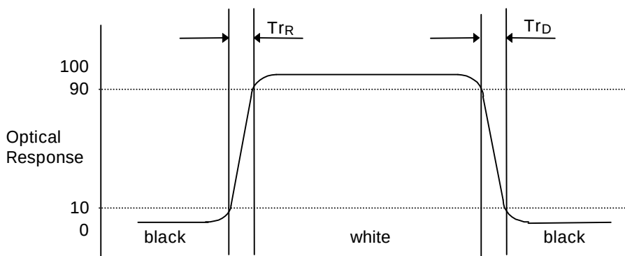
FIG. 3 Response Time
