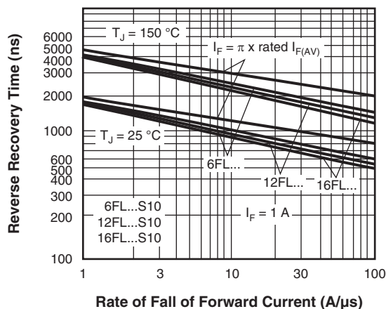
Fig. 19a - Typical Reverse Recovery Time vs. Rate of Fall of Forward Current, All Series ...S10
