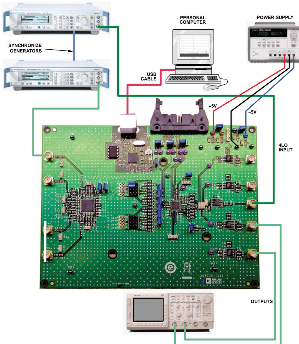
Figure 61. AD8339-EVALZ Typical Test Setup
