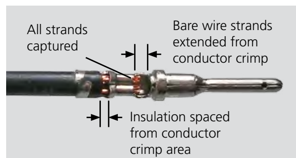
Acceptable Crimp
