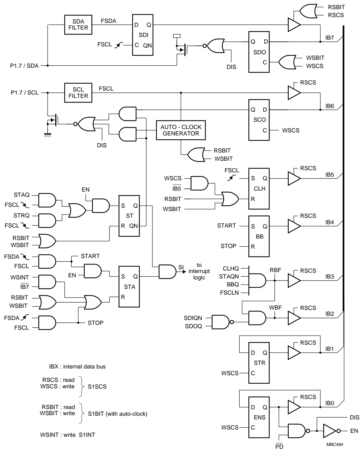
Fig.18 Bit level I²C interface block diagram.
