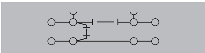
One short-circuit slider per terminal (WTL 6/1)
