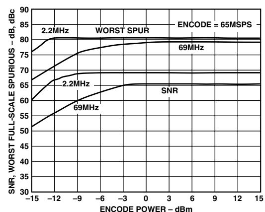
TPC 12. SNR, Worst Spurious vs. ENCODE Power
