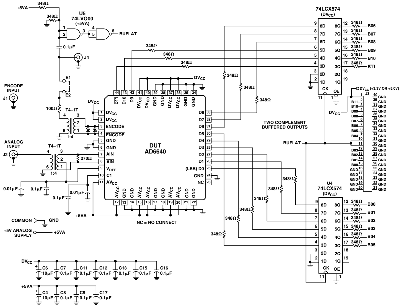
Figure 18. AD6640ST/PCB Schematic
