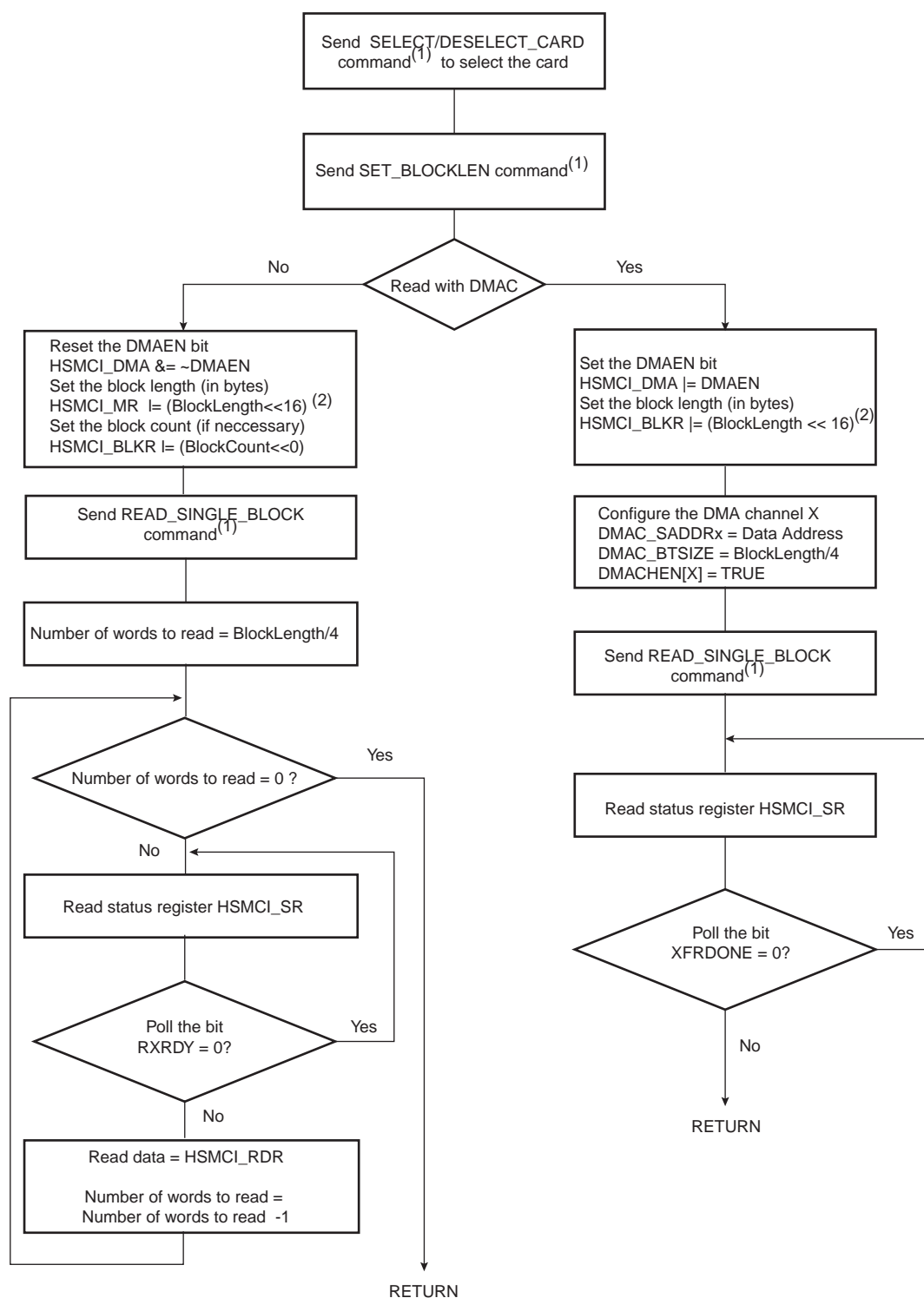
Figure 34-8. Read Functional Flow Diagram
