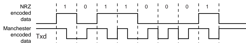
Figure 39-8. NRZ to Manchester Encoding
