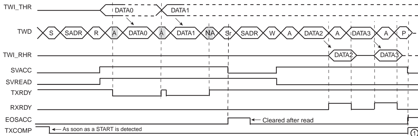
Figure 37-31.Repeated Start + Reversal from Read to Write Mode
