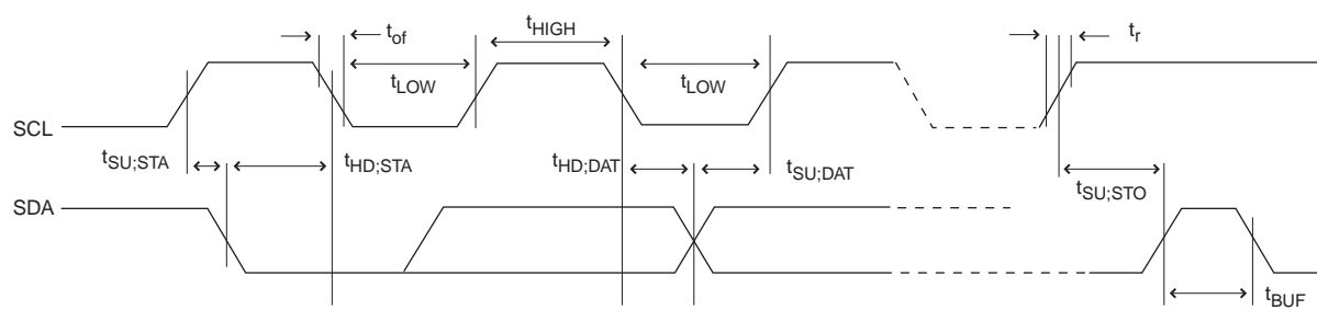
Figure 46-32. Two-wire Serial Bus Timing
