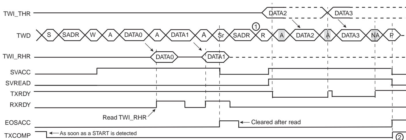
Figure 37-32.Repeated Start + Reversal from Write to Read Mode
