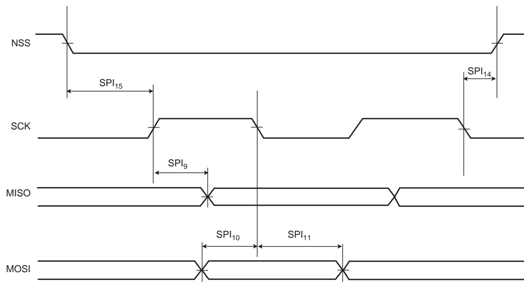
Figure 46-31.USART SPI Slave mode: (Mode 0 or 3)
