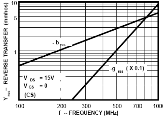
Reverse Transadmittance
