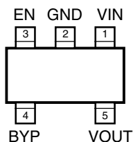
MIC5319-x.xBD5 TSOT-23-5 (D5) (Top View)
