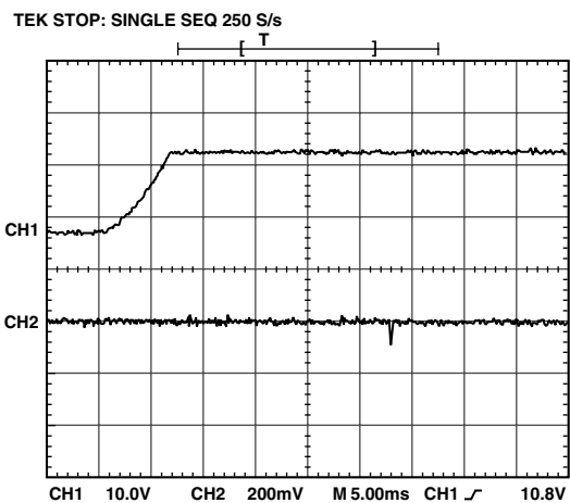
Figure 17. V_{IN} = 7.5 \text{ V to } 22 \text{ V} Transient, 2.5 V Output, CH1 – Input Voltage, CH2 – Output Voltage
