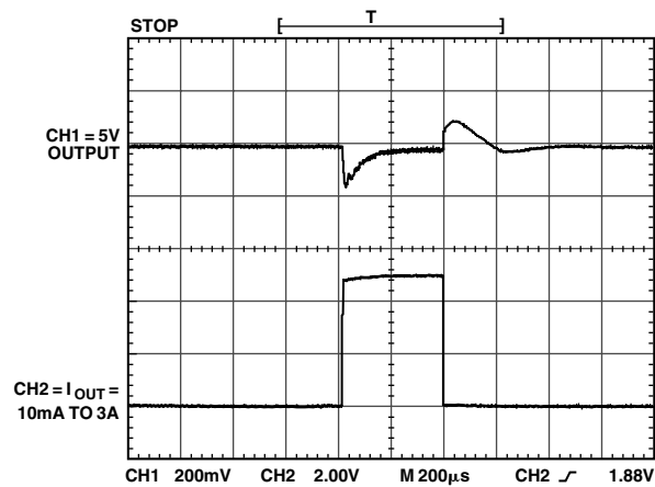
Figure 16. PWM Mode, Transient Response
