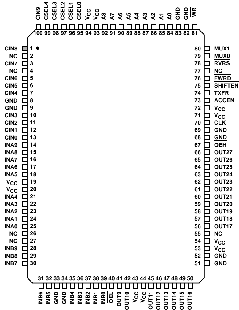
HSP43168 (100 LD MQFP) TOP VIEW
