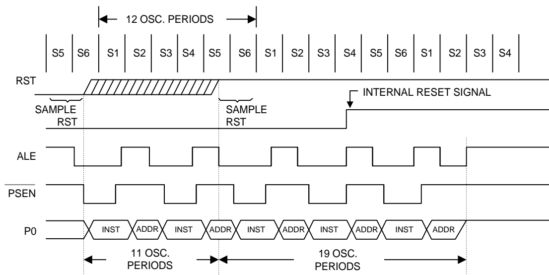
Figure 16. Reset Timing
