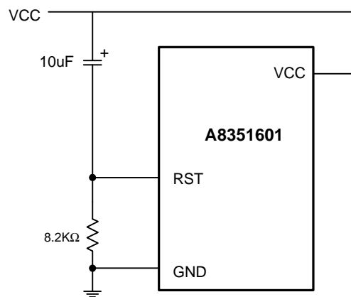
Figure 15. Power-on Reset Circuit
