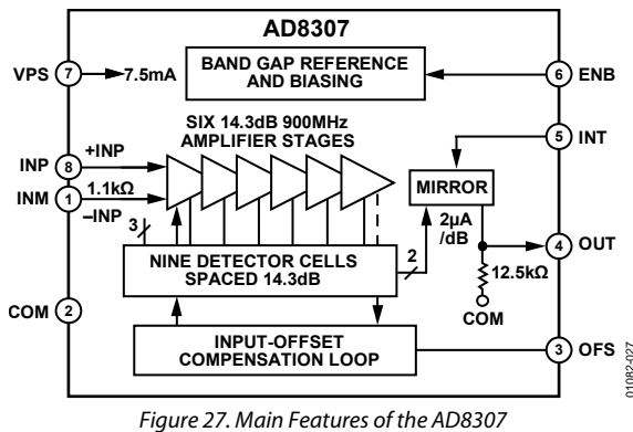
Figure 27. Main Features of the AD8307
