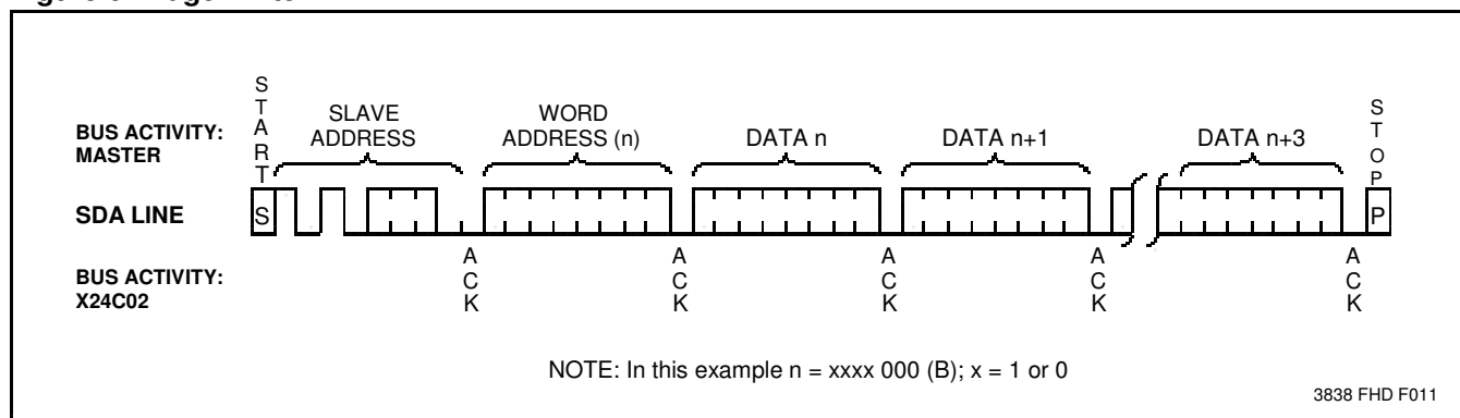
Figure 6. Page Write
