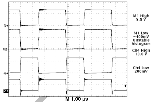
Trace 3 = V_{\text{GATE(H)}} (10 V/div.) Math 1 = V_{\text{GATE(H)}} - 5.0\text{ V}_{\text{IN}} Trace 4 = V_{\text{GATE(L)}} (10 V/div.) Trace 2 – Inductor Switching Nodes (5.0 V/div.)
