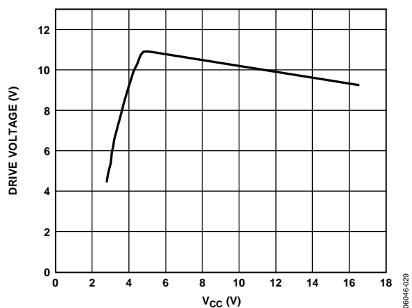
Figure 5. Drive Voltage ( V_{\text{GATE}} - V_{CC} ) vs. Supply Voltage
