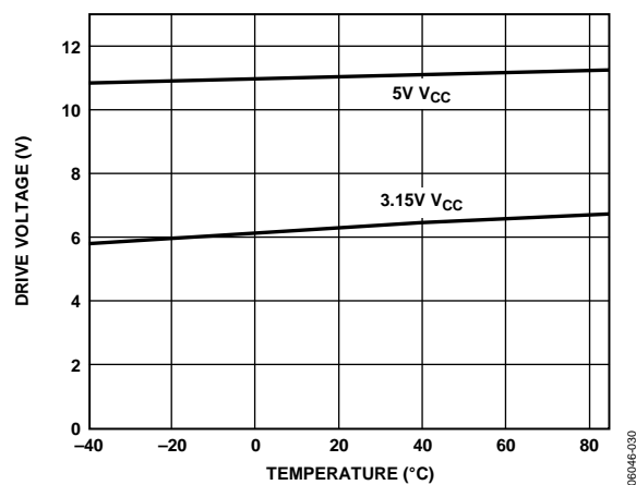
Figure 8. Drive Voltage ( V_{\text{GATE}} - V_{CC} ) vs. Temperature
